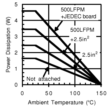
LM4873MTE (Note 20) Power Derating Curve
