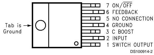
TO-220 Package Top View
