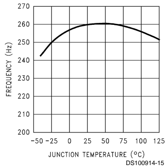
Switching Frequency
