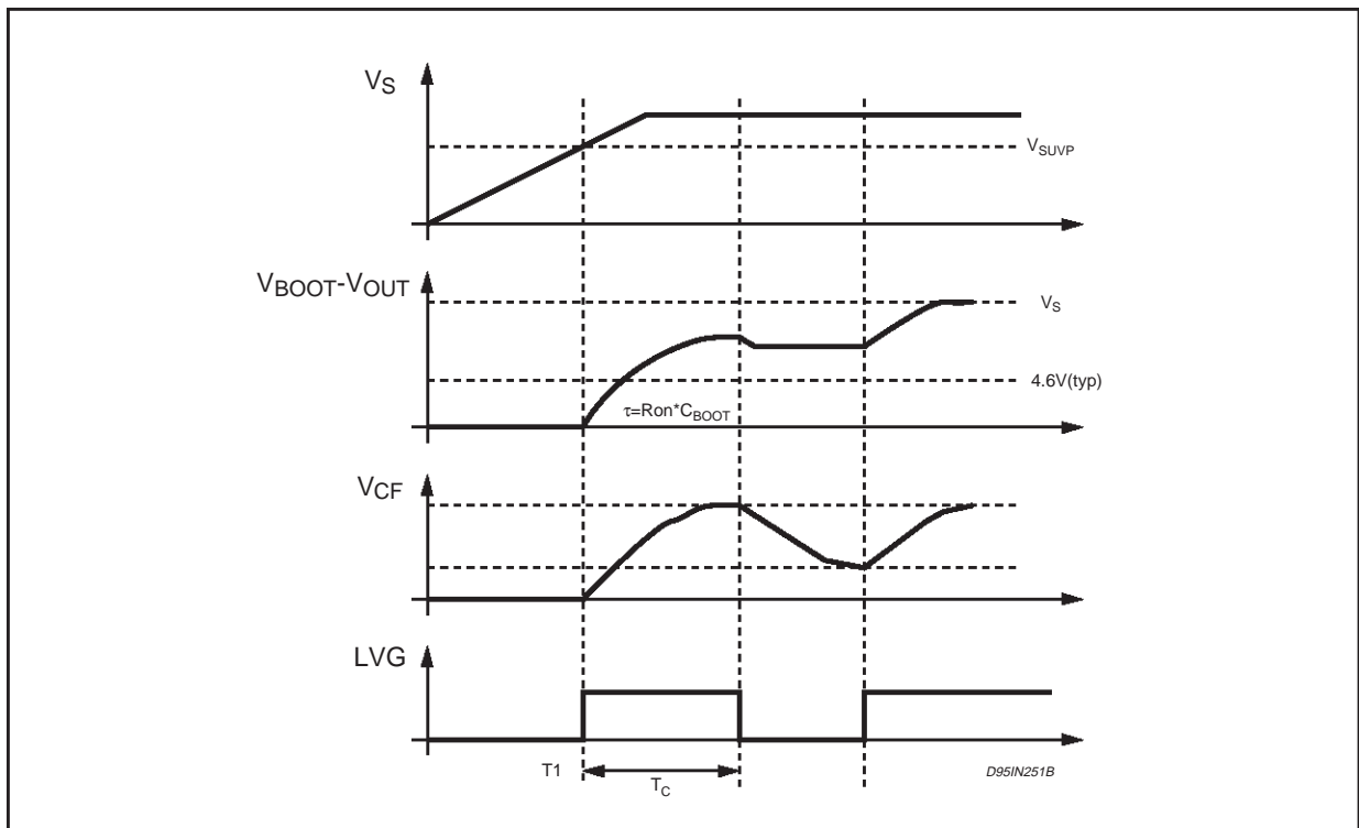
Figure 3. Waveforms (L6569A)
