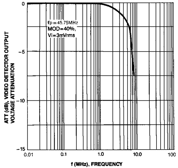
VIDEO DETECTOR OUTPUT VOLTAGE ATTENUATION Vs FREQUENCY
