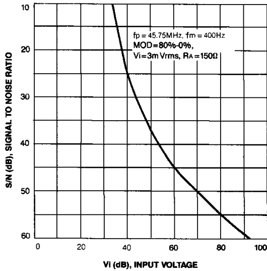
S/N Vs INPUT VOLTAGE
