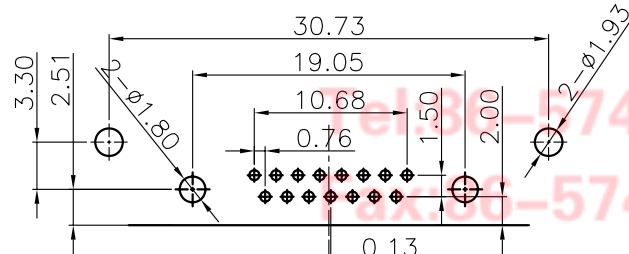
RECOMMEND PCB LAYOUT (TOLERANCE ±0.05)
