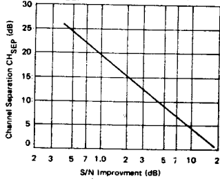
CH SEP -S/N Improvement (Graph 5)
