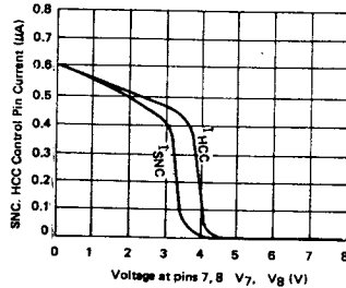
SNC, HCC Control Pin Current (Graph 6)
