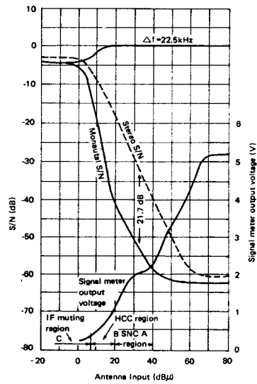
SNC and HCC Operating Regions (Graph 2)
