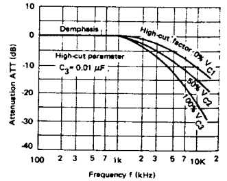
ATT-f (Graph 7)
