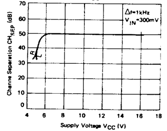
CH SEP -V CC (Graph 4)
