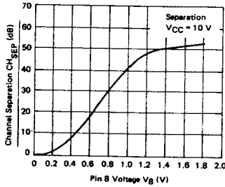
CH SEP -V 8 (Graph 3b)
