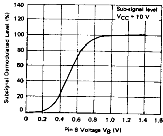
SNC Characteristics (Graph 3a)
