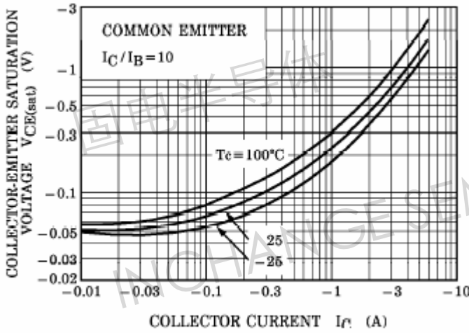
Fig.5 Collector-Emmitter Saturation Voltage
