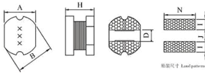
SP32 Series Dimension Diagram(unit: mm)
